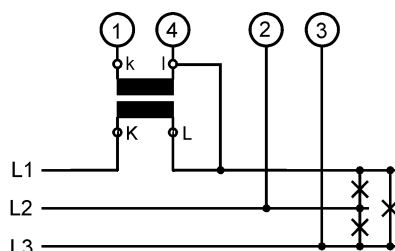
Current transformer connection
