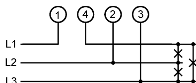
Direct access 3-phase
