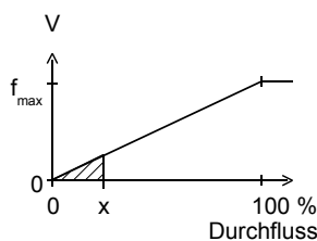
Frequenzgang
